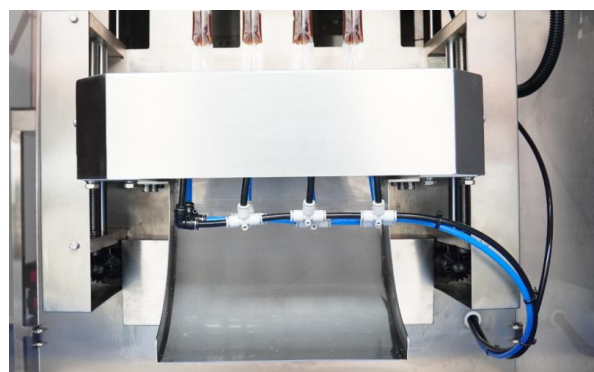
Bag making and forming+longitudinal sealing mechanism
