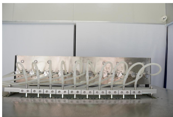
Metering system
