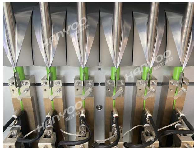
Forming mechanism
