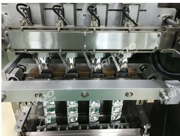
Horizontal and vertical sealing devices
